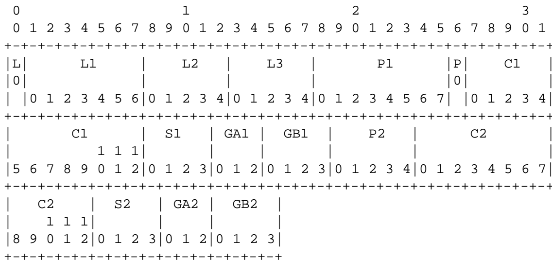
Figure 4: G.729 and G.729A bit packing
