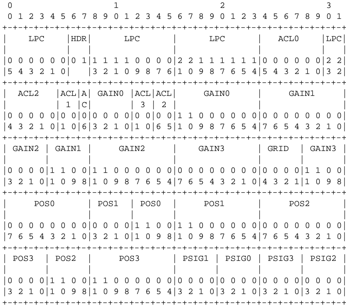
Figure 2: G.723 (5.3 kb/s) bit packing
