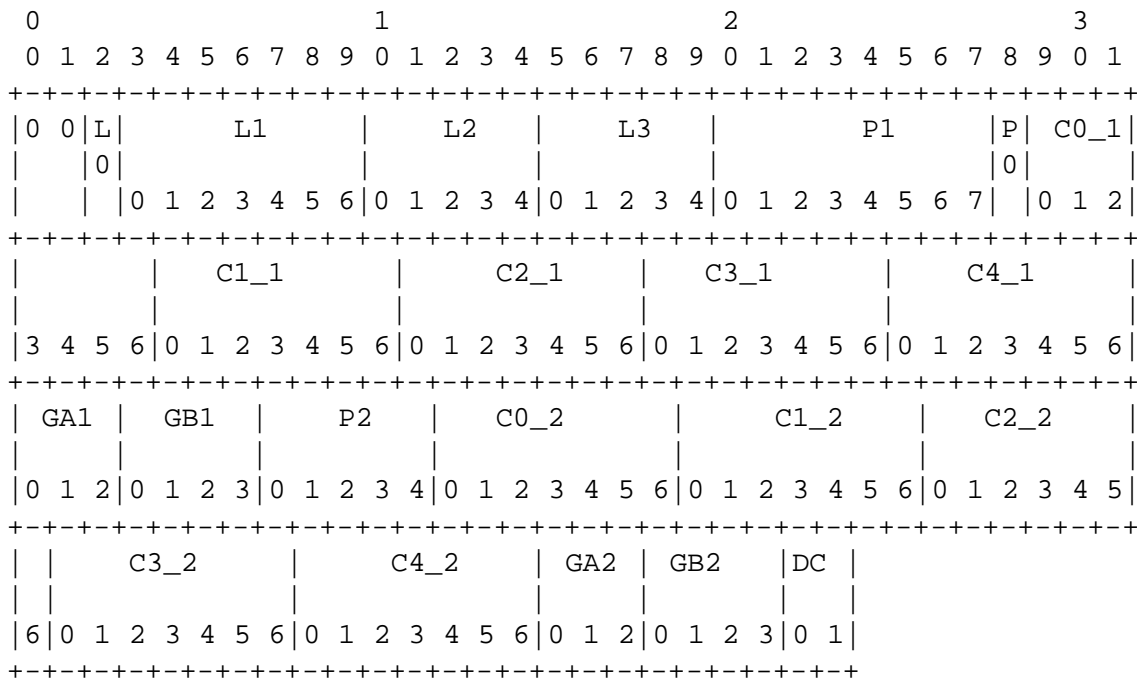
Figure 7: G.729 Annex E (forward adaptive mode) bit packing
