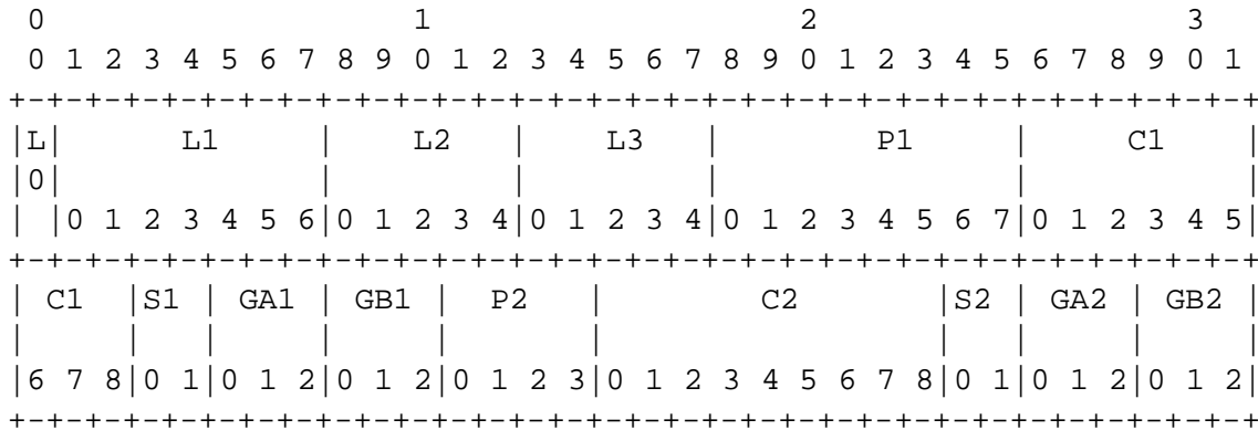
Figure 6: G.729 Annex D bit packing
