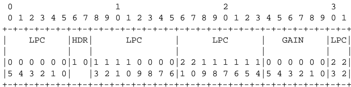
Figure 3: G.723 SID mode bit packing
