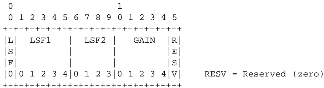
Figure 5: G.729 Annex B bit packing
