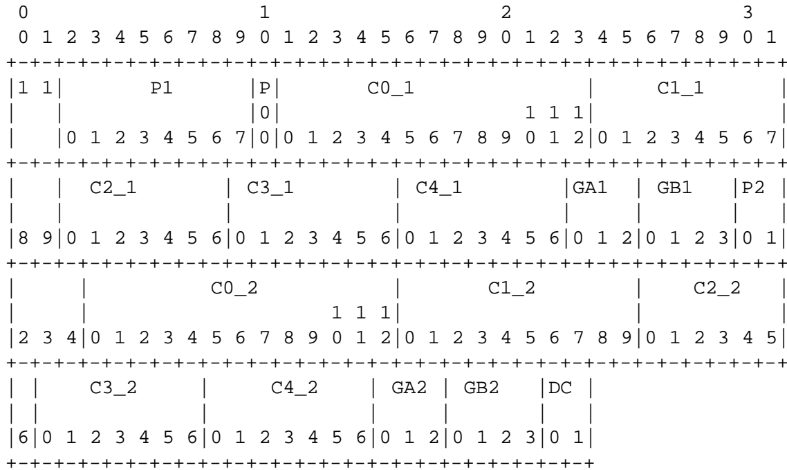
Figure 8: G.729 Annex E (backward adaptive mode) bit packing
