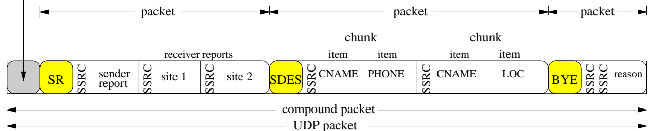
Figure 1: Example of an RTCP compound packet
