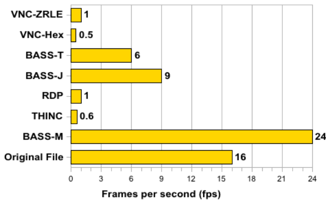
Figure 8. Movie performance (3Mb/s)
