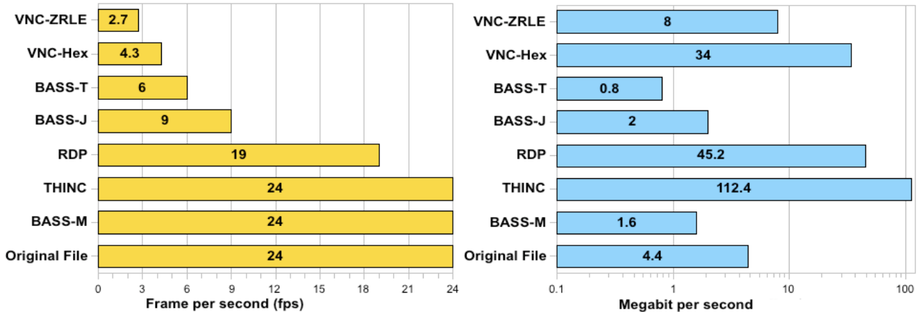
Figure 6. Comparison of sharing systems in terms of movie performance (unlimited bandwidth)
