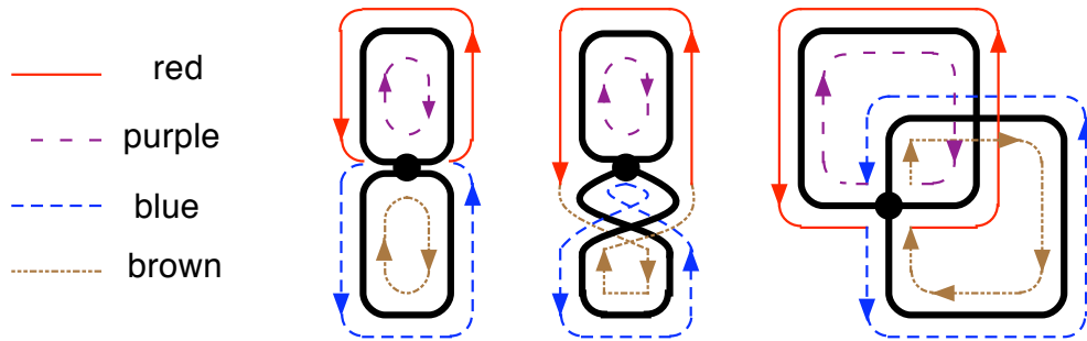
Figure 2.2: d_i * d_j \longrightarrow 4g_{i+j} + 2g_{i+j+1} .
