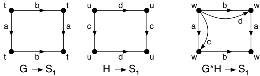
Figure 2.1: A genus increment of -1 .
