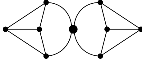
Figure 2.5: The graph X of Example 2.2.
