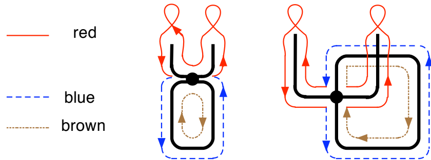
Figure 2.3: s_i * d_j \longrightarrow 6g_{i+j} .
