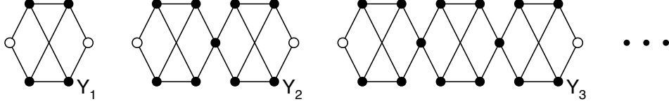
Figure 4.1: Y_n is an open chain of n copies of \ddot{K}_4 .
