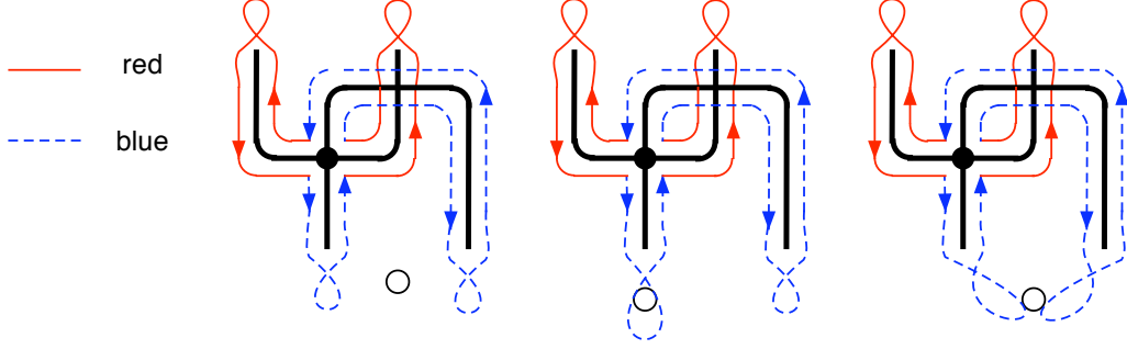
Figure 3.3: Alternating edge-ends in the three subcases of s * ss .
