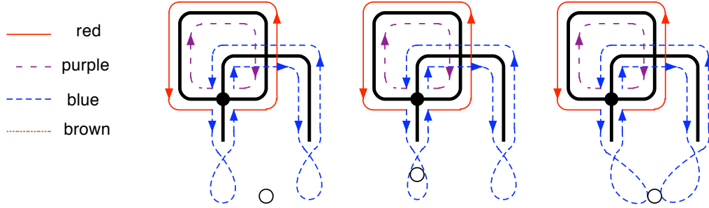
Figure 3.2: Alternating edge-ends in the three subcases of d * ss .
