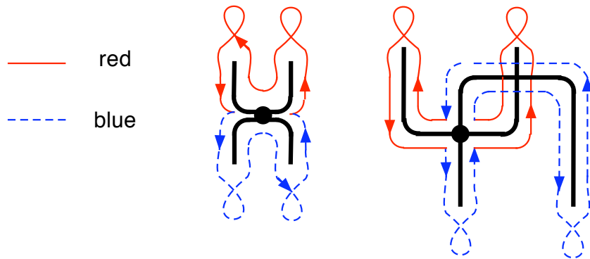
Figure 2.4: s_i * s_j \longrightarrow 6g_{i+j} .
