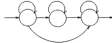
Figure 7. Topology of the HMM
