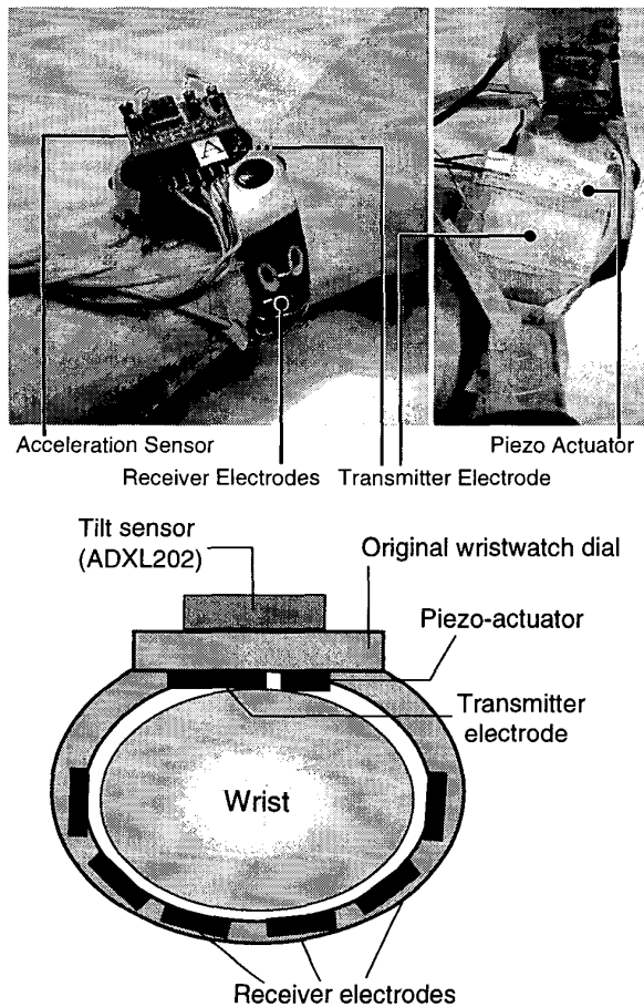
Figure 2: GestureWrist: Wristband-type input device.
