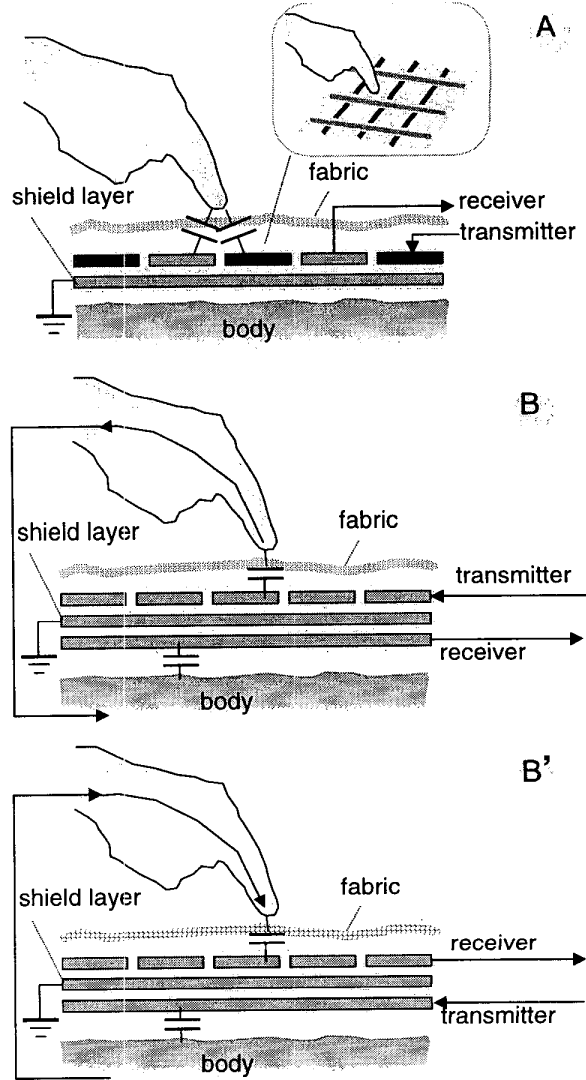
Figure 6: Sensor configurations for GesturePad
