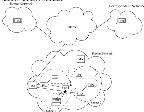
Figure 8: TeleMIP's IDMP
