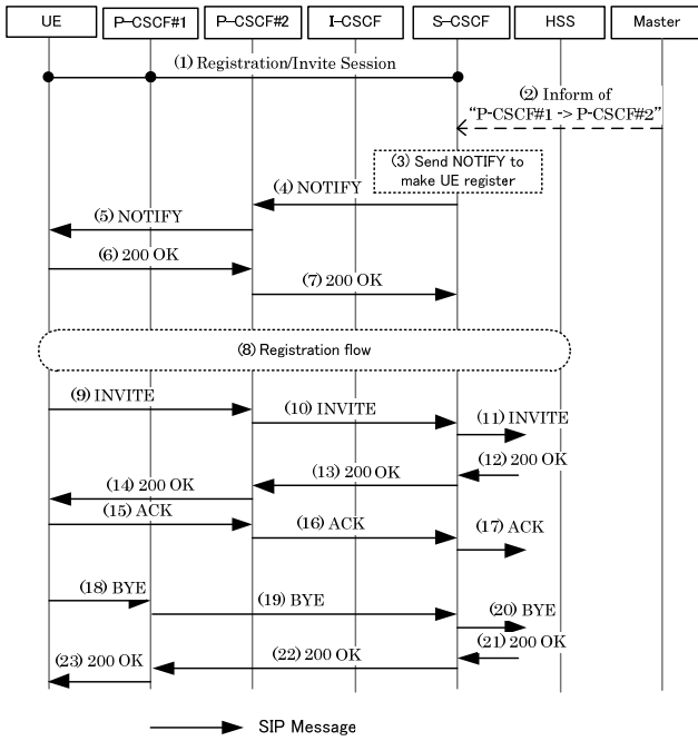
Fig. 5 P-CSCF Change Flow
