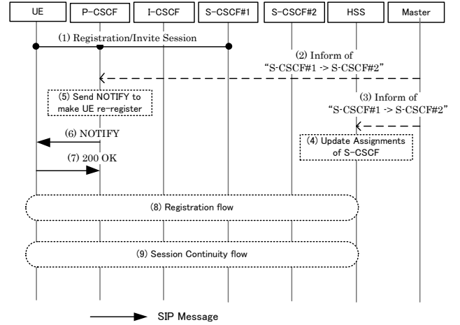
Fig. 6 S-CSCF Change Flow
