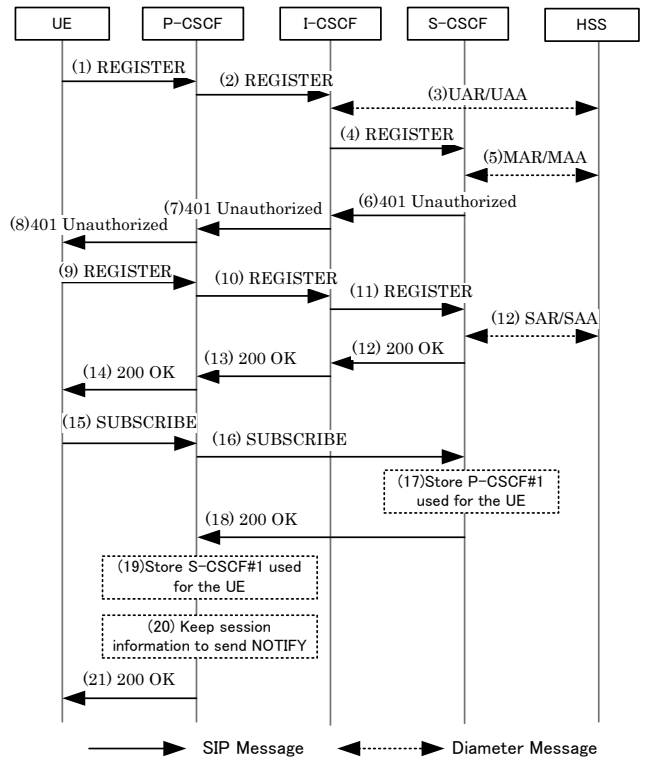
Fig. 4 Registration Flow
