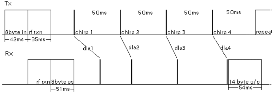
Fig. 1. Timing diagram (not to scale).
