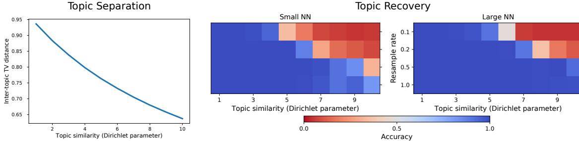
Figure 2: Topic modeling simulations. Left: Average total variation distance between topics. Right: Topic recovery accuracy for contrastive models. Total number of documents sampled = 6M \times \text{rate} .
