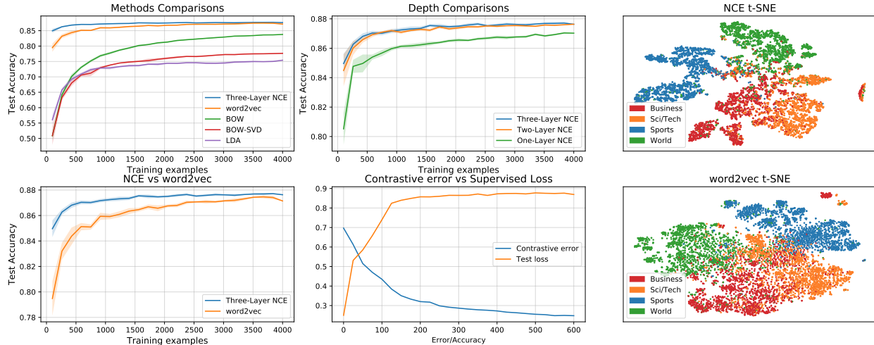
Figure 1: Experiments with AG news dataset. Left panel: test accuracy of methods as we increase the number of supervised training examples. Bottom left focuses in on NCE versus word2vec . Top middle: NCE performance as we vary network depth. Bottom middle: Relationship between contrastive error and test accuracy for NCE. Right: t-SNE visualizations of NCE and word2vec embeddings.
