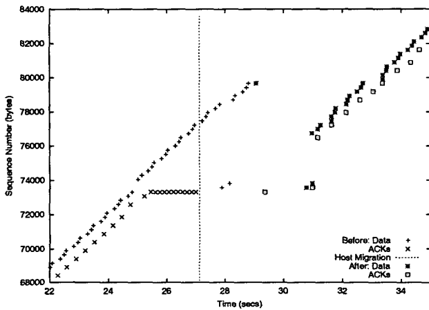
Figure 7: A TCP Migrate connection (with SACK) sequence trace with losses just before migration
