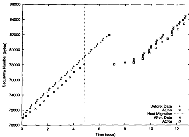
Figure 6: A TCP connection sequence trace showing the migration of an open connection
