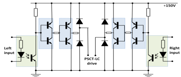
Figure 9: The PSCT-LC H-bridge driver circuit.
