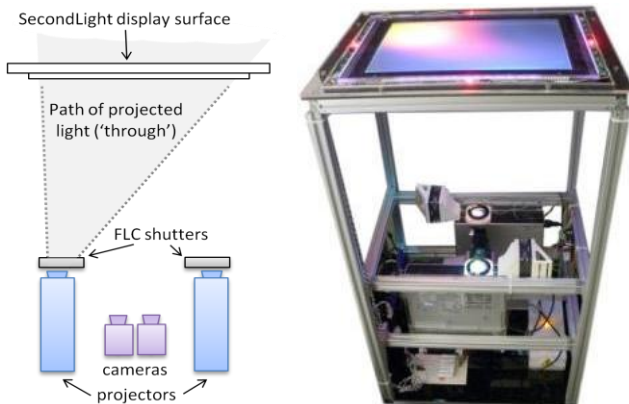
Figure 10: The layout of the main SecondLight components; on the left is a cross-section through the side of the unit and on the right is a photo from the front.
