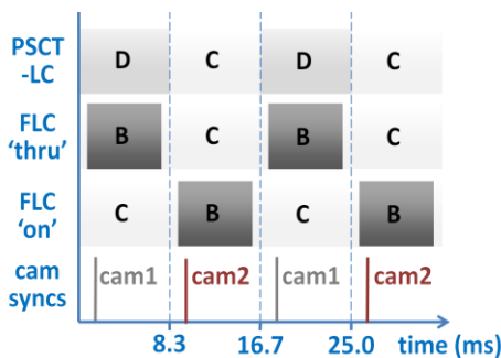
Figure 11: The timing used to drive the PSCT-LC diffuser, the FLC shutters and the camera 'sync' trigger inputs. Key: D=diffuse, C=clear, B=blocking.
