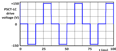
Figure 8: The waveform that drives the PSCT-LC screen. A 150V potential is applied for 8.3ms at a rate of 60Hz; to prevent any DC offset the polarity of this is reversed on alternate cycles.
