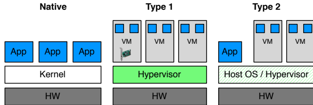
Figure 1: Hypervisor Design
