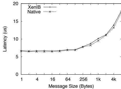
Figure 10. InfiniBand Send/Receive Latency
