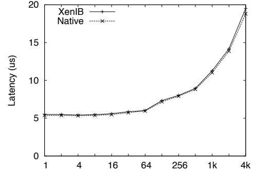
Figure 18. MPI Latency
