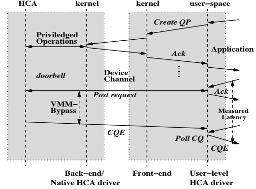
Figure 8. Working flow of the VMM-bypass Xen-IB driver
