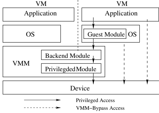
Figure 4. VM-Bypass I/O (I/O Handled by VMM Directly)
