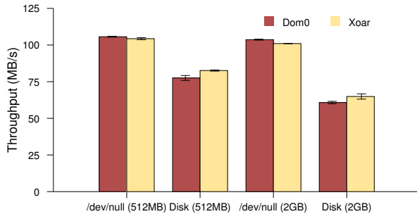
Figure 10: Network performance with wget (higher is better)
