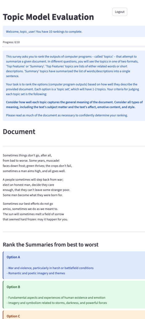
Figure 5: Screenshot of the evaluation interface shown to participants. Each task presents a document alongside topic set options produced by different models. Participants rank the options from best to worst based on how well each topic set captures the document’s meaning.
