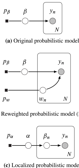
Figure 2. RPMs begin with a probabilistic model (a) and introduce a set of weights w as latent variables. This gives a model (b) that explores which data observations match its assumptions. Localization (c), instead, builds a hierarchical model. (Appendix A shows when a localized model is also an RPM.)
