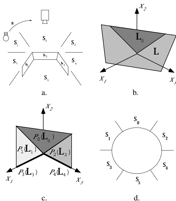
Fig. 3. A 2-D Example: a. A surface with three facets is observed from above and produces an image with pixels x_1, x_2 and x_3 . b. The linear subspace \mathcal{L} and its intersection with the positive quadrant \mathcal{L}_0 . c. The “walls” of the cone P_i(\mathcal{L}_i) corresponding to images formed by a single light source. The illumination cone \mathcal{C} is formed by all convex combinations of images lying on the walls. d. The geometry of facets leads to a partitioning of the illumination circle.
