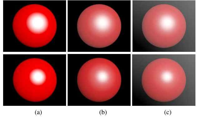
Figure 12: Influence of scattering on specular surface radiance (top row has Phong exponent 10, bottom has Phong exponent 20). In the foggy images (b), we see a dimming and diffusing of the specular highlight compared to the clear-day image in (a). Note also the overall loss in color saturation and contrast, especially in (c). These are important visual effects, usually missing in previous interactive techniques.
