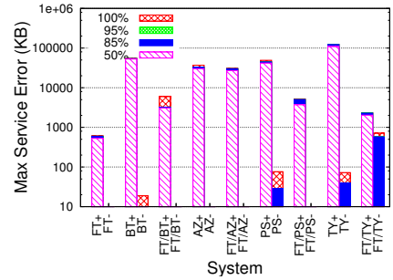
Figure 14: S: High uploader E_{\max}^+ and E_{\max}^-
