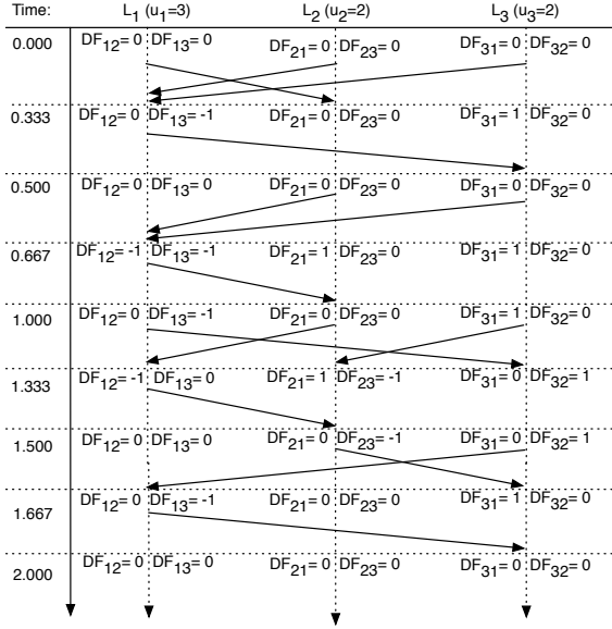
Figure 1: FairTorrent algorithm for leechers L_1 , L_2 and L_3 with upload capacities of 3, 2 and 2.
