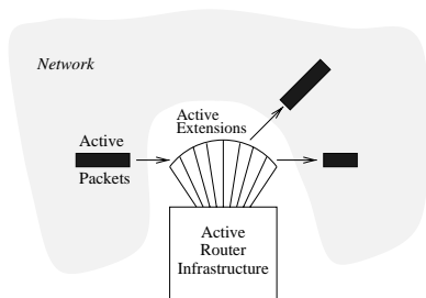
Figure 1: SwitchWare Layers
