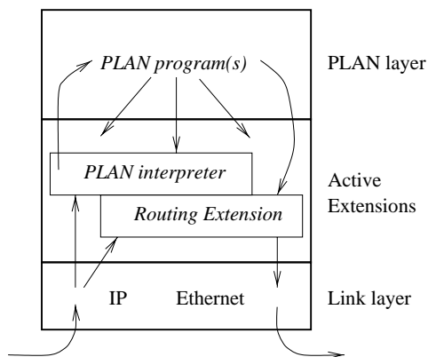
Figure 2: PLANet node architecture
