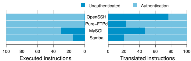
Figure 9: The percentage of instructions translated and run in the authenticated and unauthenticated partitions. The test cases we employed were: copying a 1GB file over OpenSSH , Pure-FTPD , and Samba , and the MySQL test-insert benchmark.
