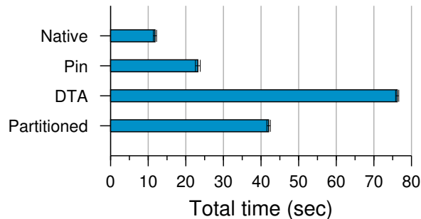
Figure 8: Time to complete MySQL’s test-ATIS benchmark. It creates 28 tables and performs a series of SELECT operations on the them. We ran the MySQL server natively, under Pin , and using DTA to track the data of a particular table ( airport ). First by applying DTA throughout the benchmark, and then by partitioning execution and activating it only after data are read from the table (labeled as Partitioned ).
