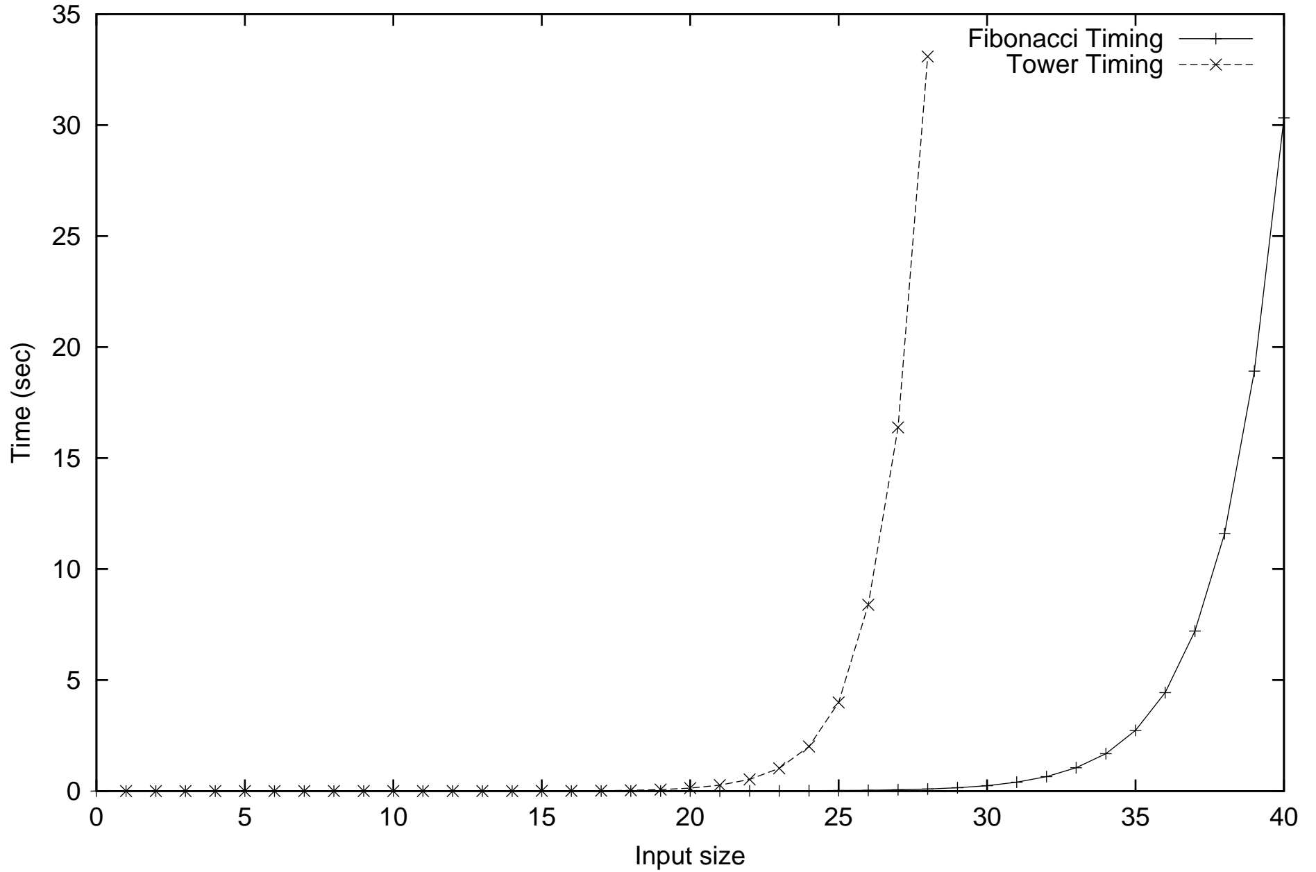
Running Time of Fib and Tower Calculation
