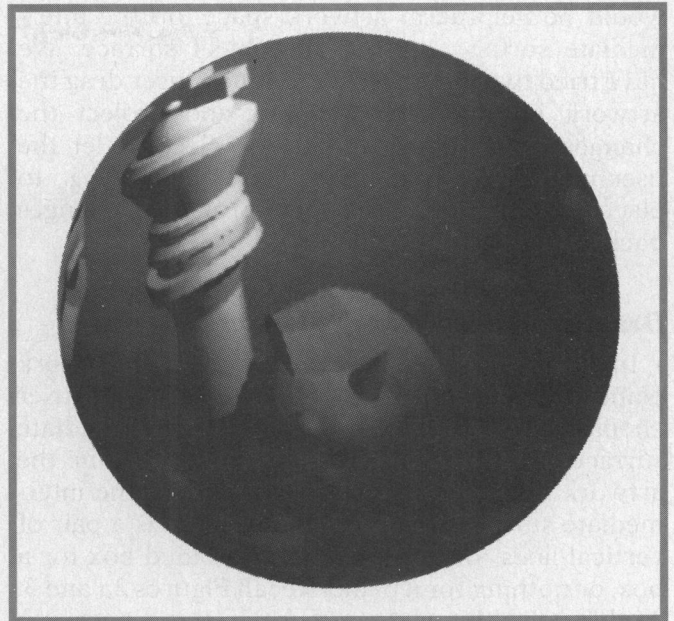
Figure 12. ISN/box mapping applied to the chess scene. The side of the simple surface cube is \sqrt{2}/2 times the diameter of the sphere. This cube size minimizes the amount of data lost, given that all sphere points are to receive color from the texture pattern. The distortion is hard to perceive.
