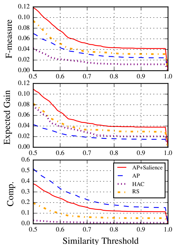
Figure 4: Expected Gain and Comprehensiveness performance.
