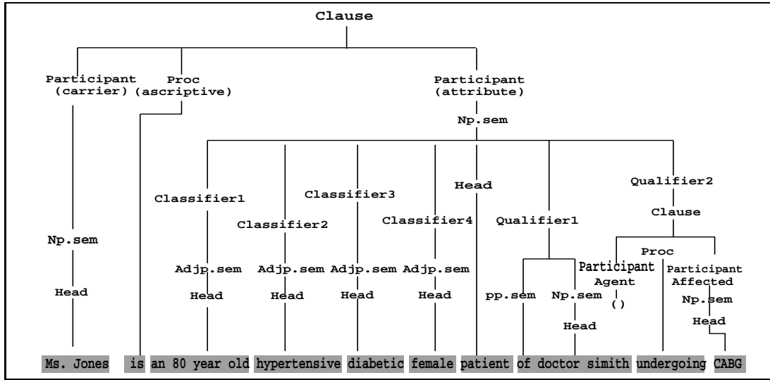
Figure 2: Semantic Structure and BSU
