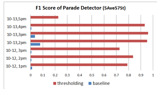
Figure 8: F1 Score for Camera in 5 Avenue at 57 Street
