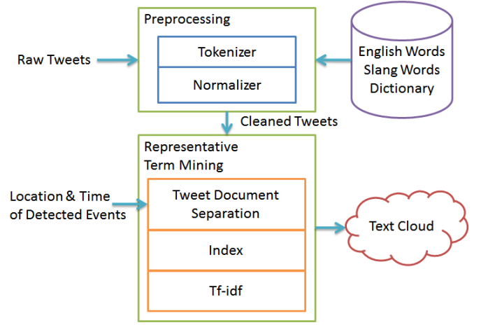
Figure 4: Architecture of Twitter Data Processing.
