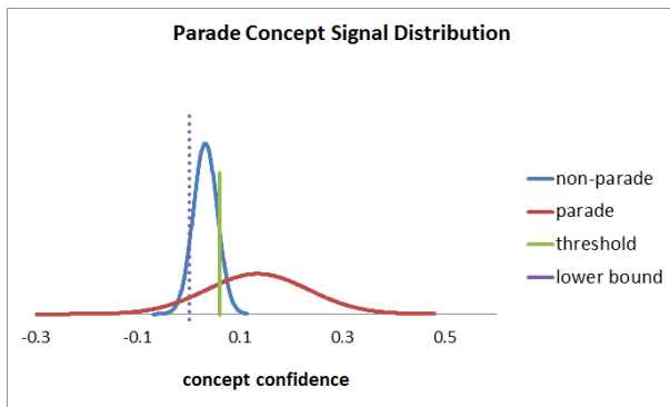
Figure 5: “Parade” Signal Distribution in 5 Ave @ 57 Street.
