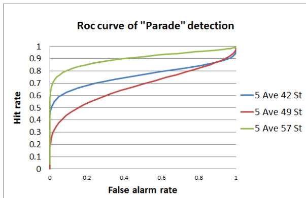
Figure 6: ROC Curve of “Parade” Signal in Three Locations.
