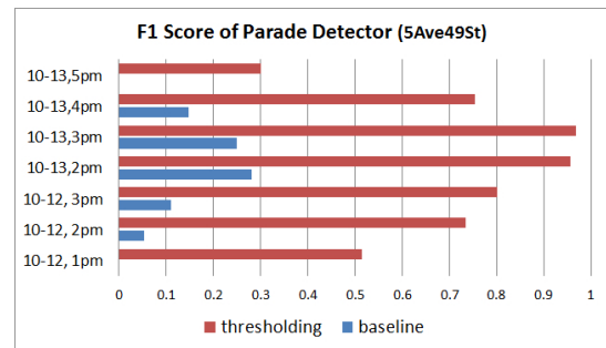
Figure 7: F1 Score for Camera in 5 Avenue at 49 Street
