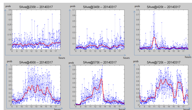
Figure 9: People Marching Concept Results from 8:00 to 18:00 in March 17th, during Saint Patrick’s Day Parade Event
