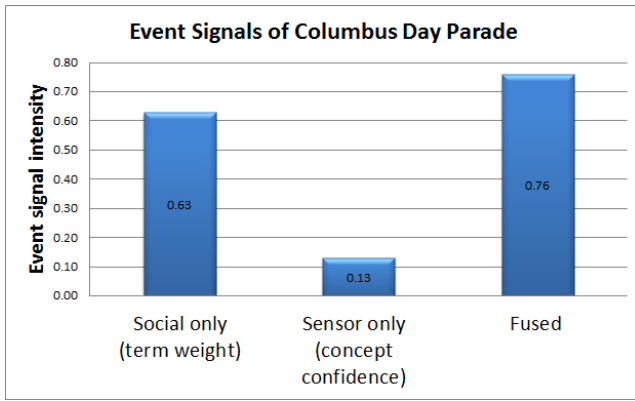
Figure 13: Comparison among Fused, Physical and Social Sensor Results of Detecting the “Columbus Day Parade” Event
