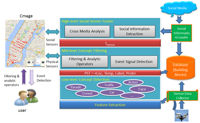
Figure 2: Overview of Proposed Multi-layer Tweeting Cameras Framework. In the first layer, low-level concepts are detected from raw sensor images through applying various concept detectors. A unified probabilistic spatio-temporal (PST) data structure represents the low-level concepts. Those camera “tweets” of low-level concepts are then aggregated and processed at the second layer using a set of predefined operators and functions. Signal detection theory is applied to detect abnormal patterns indicating occurring events. In the third layer, social information and the processed camera tweets are fused to derive high-level semantics.
