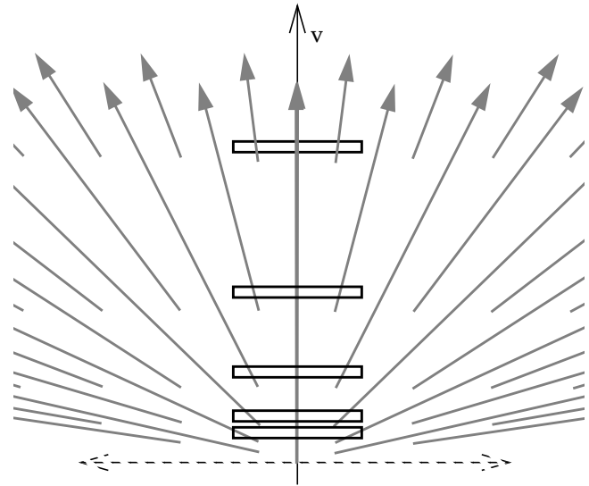
Figure 12. Fractal grid in 1D. As the window moves up by a factor of 2 magnification, new gridpoints appear to subdivide the world appropriately at that scale. The view of the grid is the same in all five windows.
