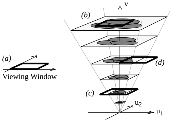
Figure 2. The viewing window (a) is shifted rigidly around the 3D diagram to obtain all possible pan/zoom views of the original 2D surface, e.g., (b) a zoomed in view of the circle overlap, (c) a zoomed out view including the entire original picture, and (d) a shifted view of a part of the picture.
