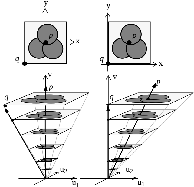
Figure 4. Shear invariance. Shifting the origin in the 2D picture from p to q corresponds to shearing the layers of the diagram so the q line becomes vertical. Each layer is unchanged, and great rays remain straight. Only those conclusions which remain true under all such shears are valid.
