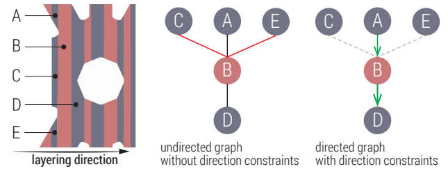
Fig. 8. Graph construction and traversal. (left) We identify individual pixel regions (A-E) through flood filling. (middle) We create a graph, where each node represents a pixel region, and two nodes are connected if their regions are adjacent to each other. Since the layers are added along the printing direction, it makes no sense to traverse back and forth along the printing direction for decoding—for example, A \rightarrow B \rightarrow C does not produce a valid bit string, while A \rightarrow B \rightarrow D is reasonable (right).
