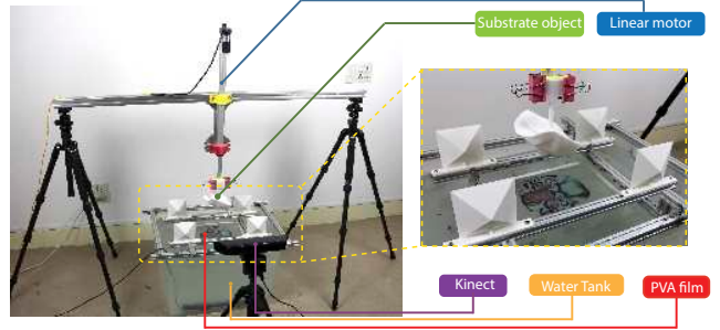
Figure 8: System setup. Our hydrographic printing system consists of a vat filled with water to hold the color film, a linear motor to drive a mechanical gripper that holds the substrate object, and a Kinect for measuring the object’s orientation and dipping location.
