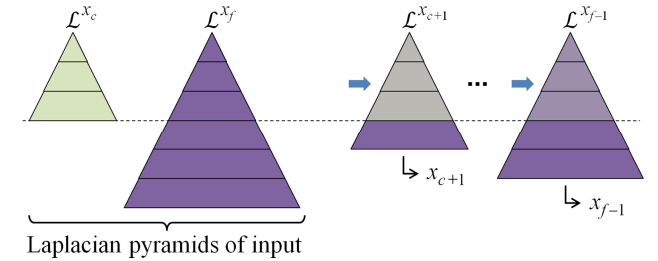
Figure 10: Clipped Laplacian blending creates intermediate-resolution images by smoothly transitioning coarse levels of the Laplacian pyramids while iteratively adding intact fine detail.
