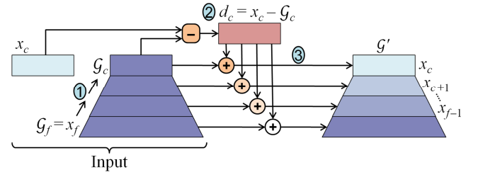
Figure 11: Equivalent efficient blending algorithm with 3 simple steps: (1) downsampling to form Gaussian pyramid, (2) coarse-level differencing, and (3) fading the difference into the pyramid.
