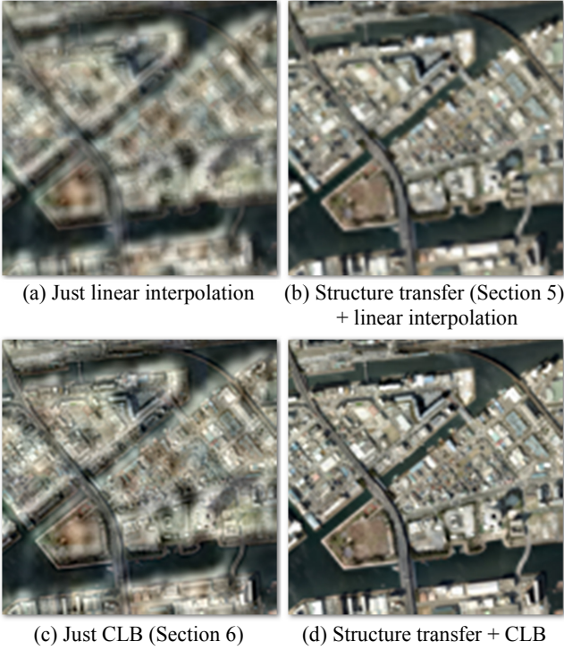
Figure 6: Close-ups comparing the blended images at 256^2 resolution obtained with different interpolation strategies, using the input images of Figure 1. Structure transfer reduces ghosting, and clipped Laplacian blending (CLB) reduces blurring.
