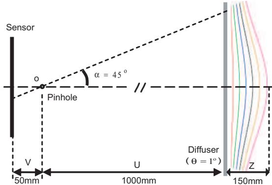
Figure 4. Equi-diffusion surfaces of a simulated pinhole camera with a diffuser. Six equi-diffusion surfaces (1D) are shown in different colors.
