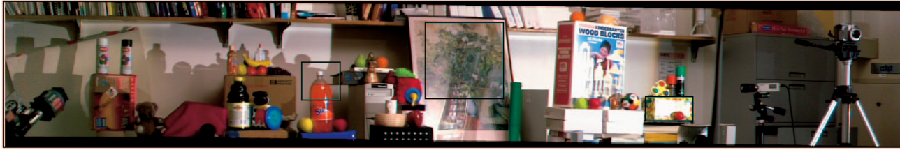
Fig. 5. The image mosaic rendered based on the frames acquired via the spatially varying filter. This is the image of the estimated unpolarized component c . The marked areas are analyzed as described in Section 5.3.
