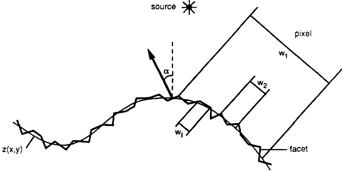
Figure 1: Rough Surface.
