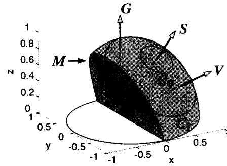
Figure 1. The surface normal set C_o is the cone satisfying \{n : n \cdot S = I_o\} , where S is the illumination or source direction. Similarly C_1 is the cone satisfying \{n : n \cdot S = I_1\} . The set M of surface normals satisfying (n \cdot V > 0) and (n \cdot G > 0) is illustrated by the partial sphere. Notice that C_o \cap M is the entire cone while C_1 \cap M is a portion of the cone.
