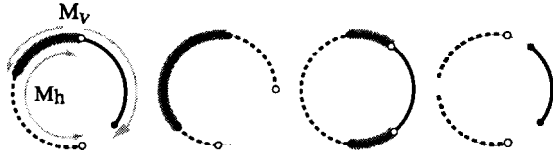
Figure 6. From left to right, the four main intersection outcomes M_v \cap M_h are illustrated: (1) the sets partially overlap, (2) one set is a subset of the other, (3) the intersection is two disjoint sets, and (4) the intersection is the empty set. In each illustration, the solid line terminated by solid circles corresponds to M_v , the dashed line terminated by open circles corresponds to M_h and the wide gray line corresponds to the intersection.
