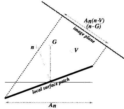
Figure 2. Foreshortening geometry. A section of the surface with normal n and area A_n is projected to an image region with area \frac{A_n(n \cdot V)}{(n \cdot G)} . This geometry is used to derive the foreshortening factor.
