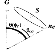
Figure 5. The cone illustrated corresponds to the surface normals for intensity I_o according to the Lambertian assumption. In the coordinate frame aligned with the illumination direction S , these surface normals have the same polar angle \theta_{co} but different azimuth angles \phi_c . A given surface normal n_c makes an angle of \theta(\phi_c) with the global surface normal G .
