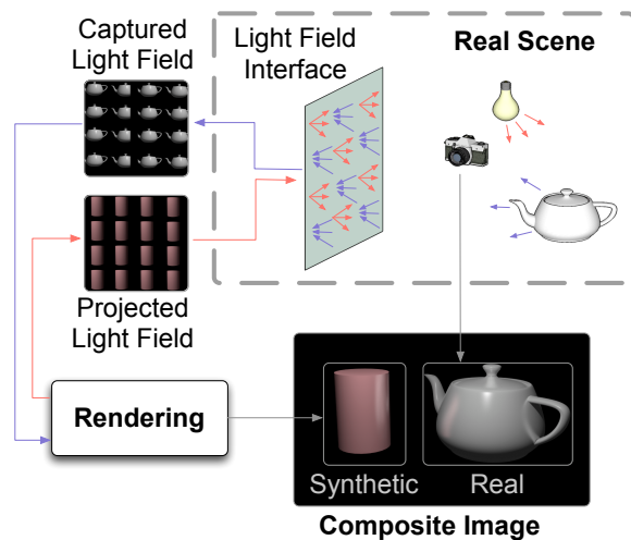
(a) Dataflow for light field transfer
