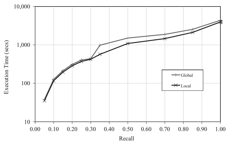
Fig. 25. Actual execution times for the “global” and “local” optimization approaches, for Task 1b and as a function of the target recall \tau .
