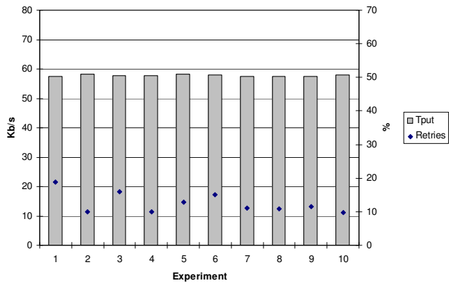
Fig. 6. Throughput and retry rate with interference on channel 4
